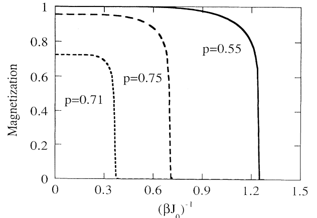
FIG. 1. Magnetization vs temperature for the two-dimensional nonequilibrium impure (solid line) and spin-glass models (dashed lines) for different p values.
